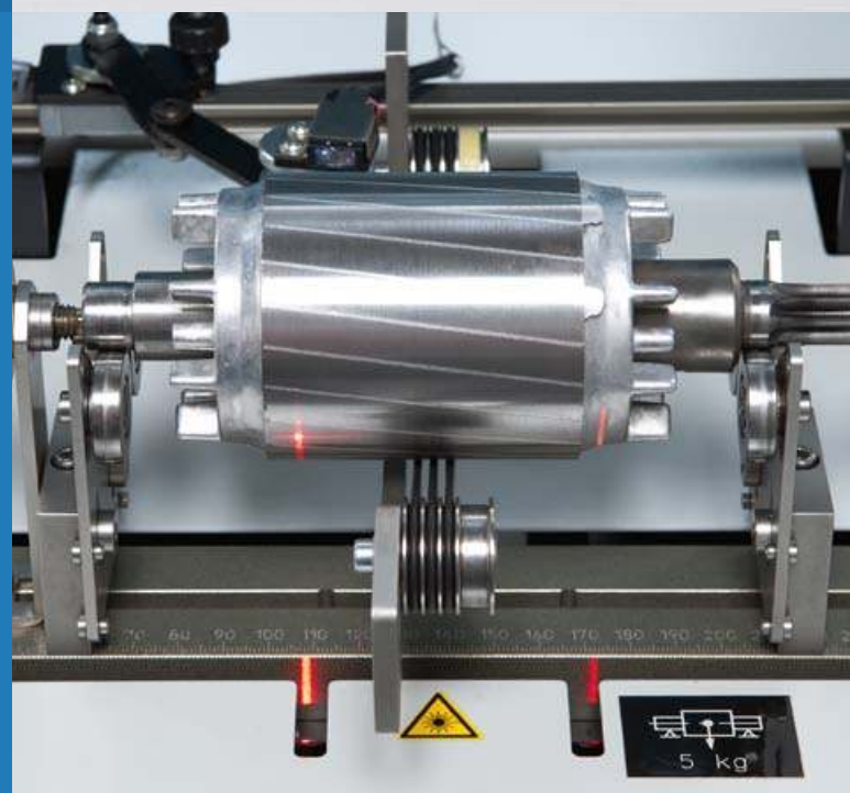
The line laser ensures the clear display of the measurement planes (Pasio 5)
